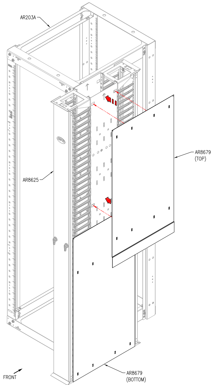
AR8625 CABLE MANAGER SHOWN w/ AR203A OPEN FRAME RACK
