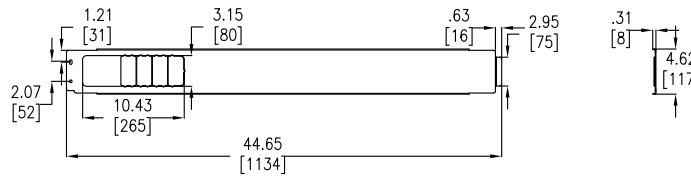
PART "F" – FRONT VIEW
