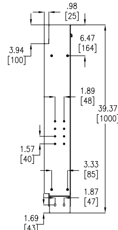
PART "K" - FRONT VIEW
