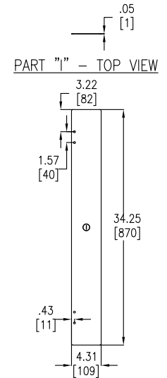
PART "I" - TOP VIEW
