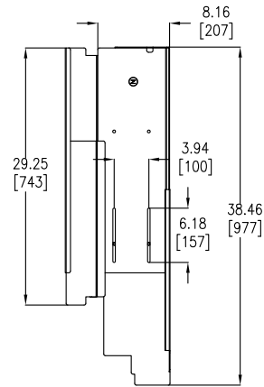
PART "N" (ASSEMBLED) - TOP VIEW
