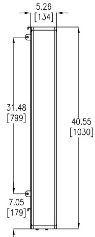
PART "D" – FRONT VIEW
