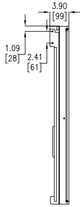
PART "A" – SIDE VIEW
