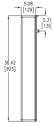
PART "C" – FRONT VIEW
