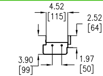
PART "B" – TOP VIEW
