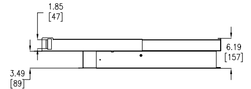
PART "N" (ASSEMBLED) - SIDE VIEW
