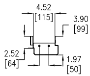
PART "D" – TOP VIEW
