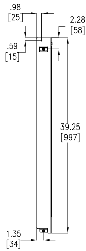
PART "J" - SIDE VIEW
