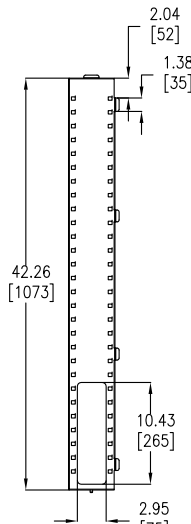
PART "L" - TOP VIEW
