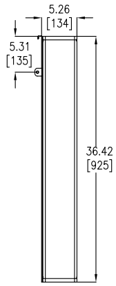
PART "A" – FRONT VIEW
