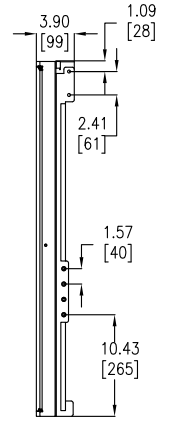
PART "C" – SIDE VIEW
