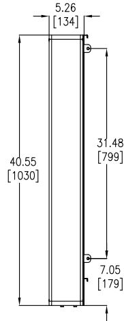
PART "B" – FRONT VIEW
