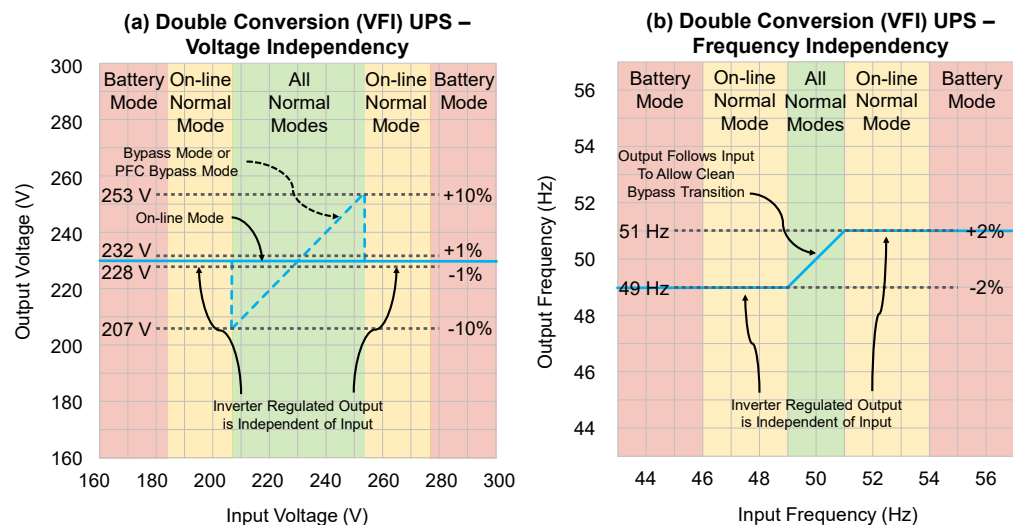
Figure A4 (a) and (b) Examples of output voltage and frequency independency for a double conversion (VFI) UPS
