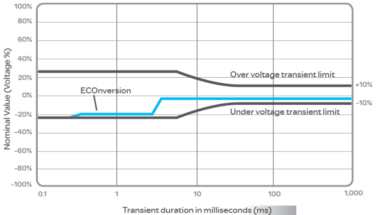
Figure 10: In EConversion mode the UPS is rated as a class 1 system giving zero breaks transfer at power outage (ICE 62040-3).
