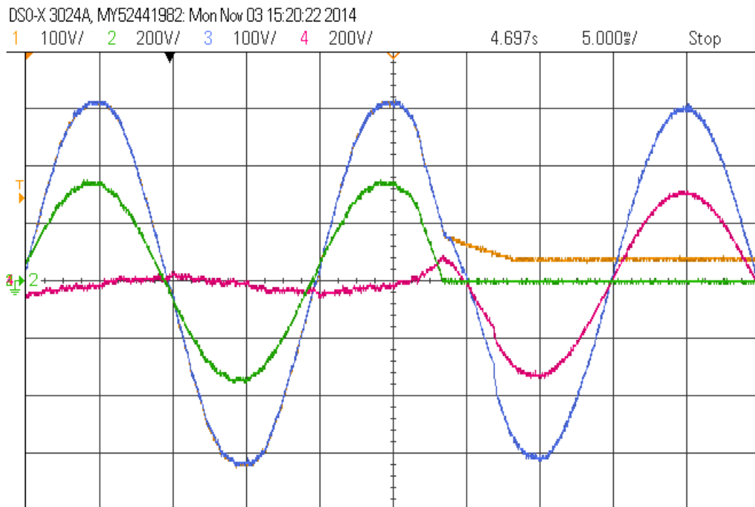
Figure 4: Situation with 95% ohm load applied on a 4-wire 400 V 50 Hz system.
