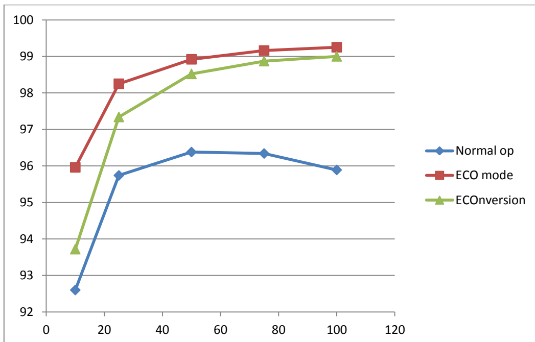
Figure 15: Efficiency plot data derived from Table 2
