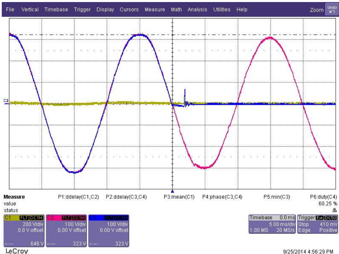
Figure 8: Upstream short when systems in EConversion Mode 0% load short at 180 degrees.
