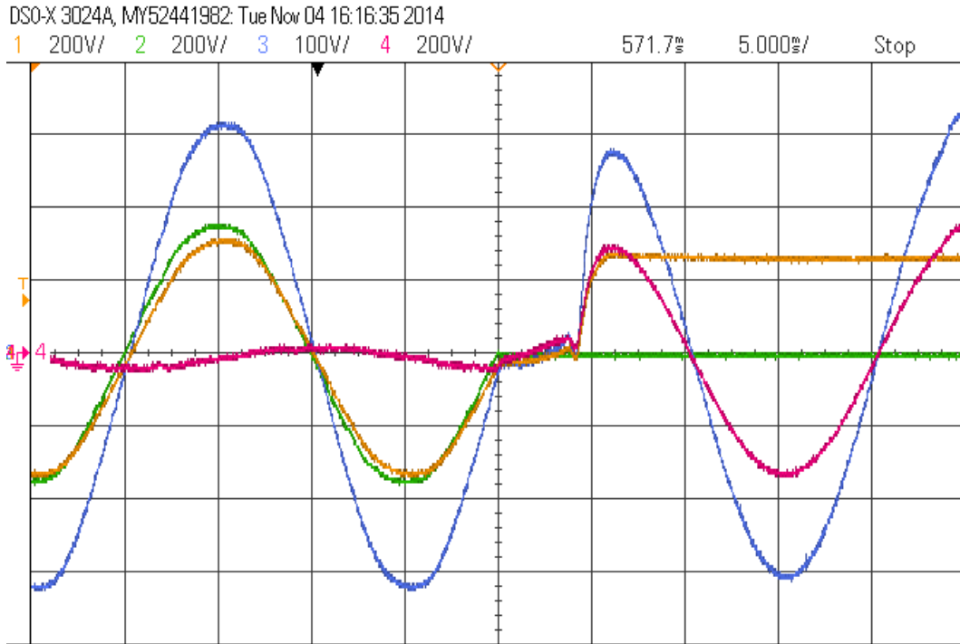
Figure 5: Situation with 95% ohm load applied on a 4-wire 400 V 50 Hz system. Blue Inverter V, Red Inverter I, Yellow Bypass V, Green Bypass I
