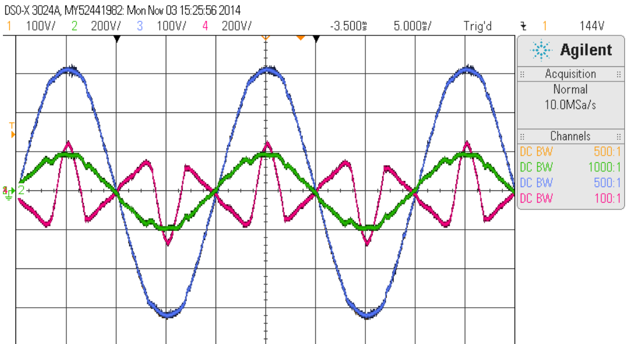
Figure 14: Situation with 60% SMPS load applied on at 4-wire 400 V 50 Hz system. Blue Inverter V, Red Inverter I, Yellow Bypass V, Green Bypass I
