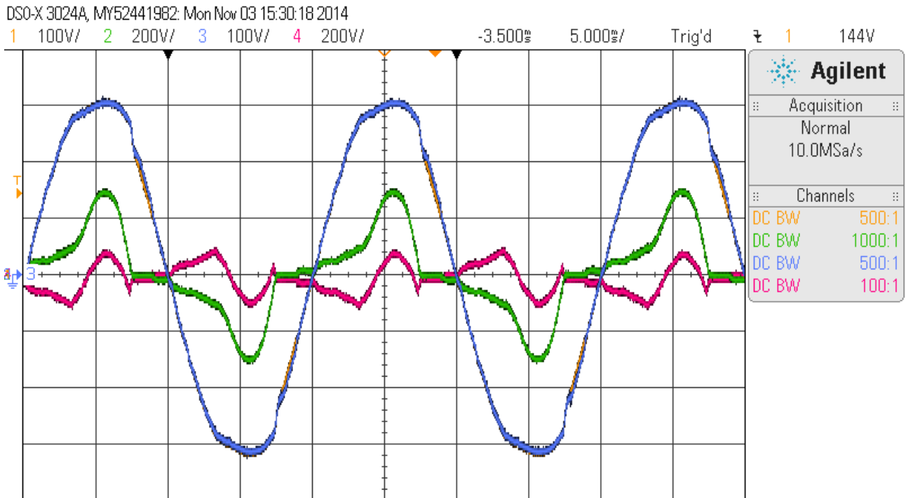
Figure 13: Situation with 60% SMPS load applied on at 4-wire 400 V 50 Hz system. Blue Inverter V, Red Inverter I, Yellow Bypass V, Green Bypass I
