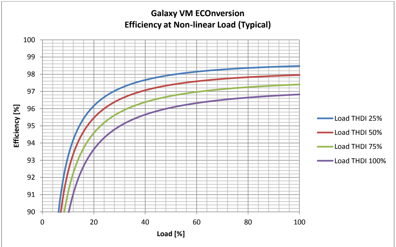
Figure 19: System efficiency relate to harmonic content.
