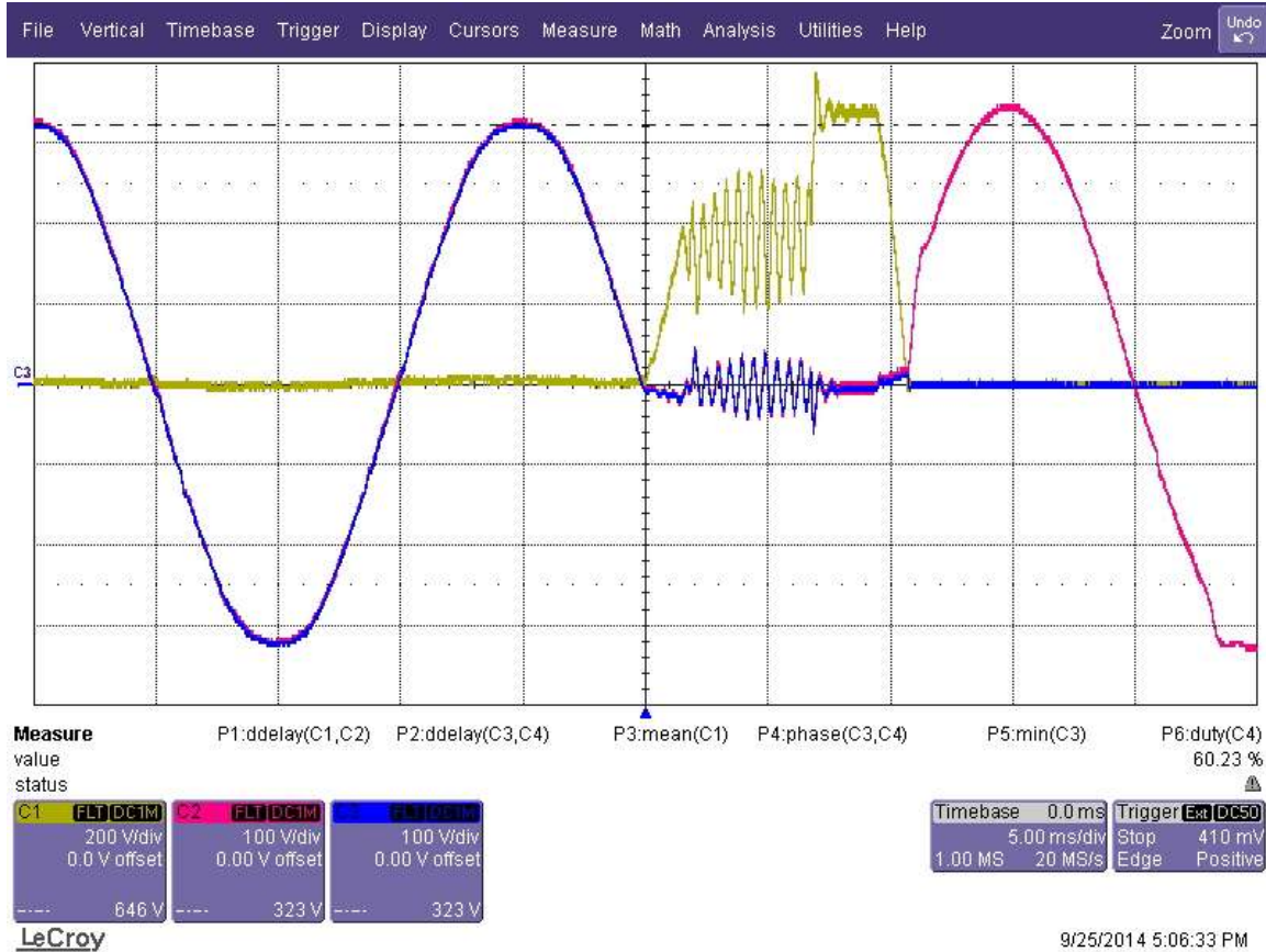
Figure 9: Upstream short when systems in ECO Mode 0% load short at 180 degrees. Blue bypass V, yellow bypass I, red inverter V,
