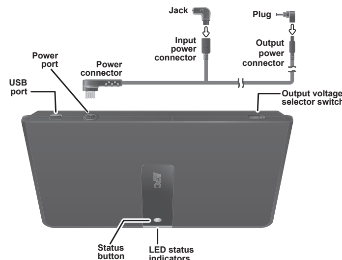
Figure 1: Components
